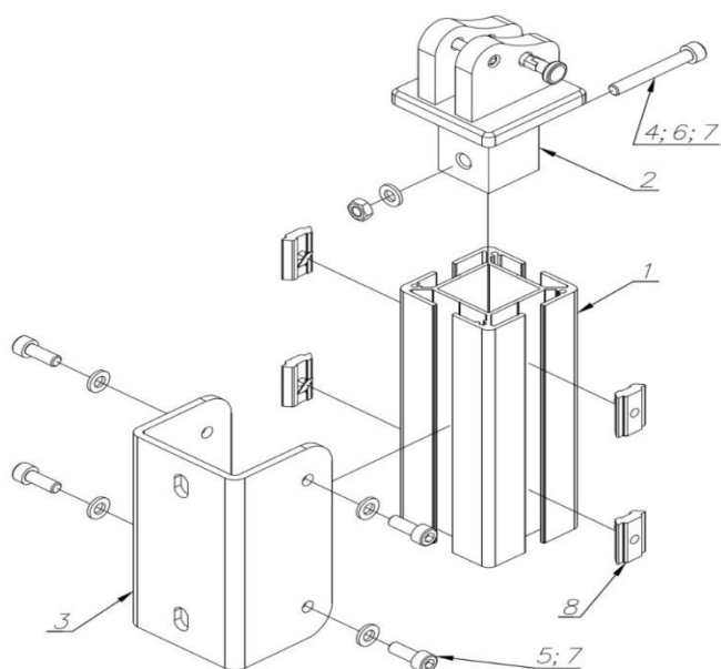
Support mural fixe
